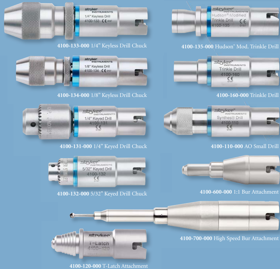
4100-120-000 T-Latch Attachment
